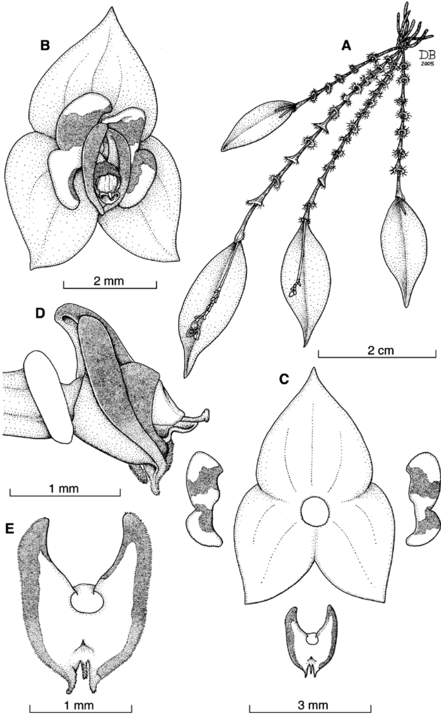
FIG. 2. Lepanthes dikoensis Bogarín & C.M. Sm. A) Habit. B) Flower. C) Dissected perianth. D) Column and lip, lateral view. E) Lip, spread. Drawn by D. Bogarín from the holotype (JBL-Spirit).
